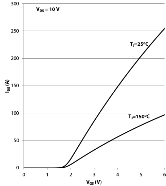
GS61008T I_{DS} vs. V_{GS} Characteristic
