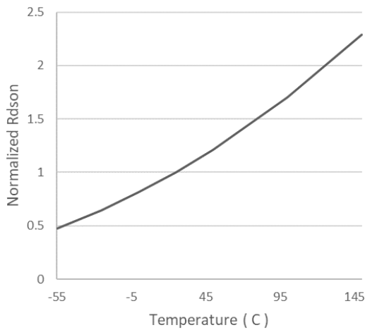
GS61008T R_{DS(on)} Temperature Dependence R_{dson}(T)
