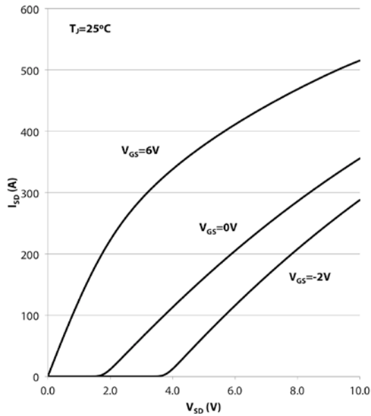
GS61008T Reverse Conduction Characteristics
